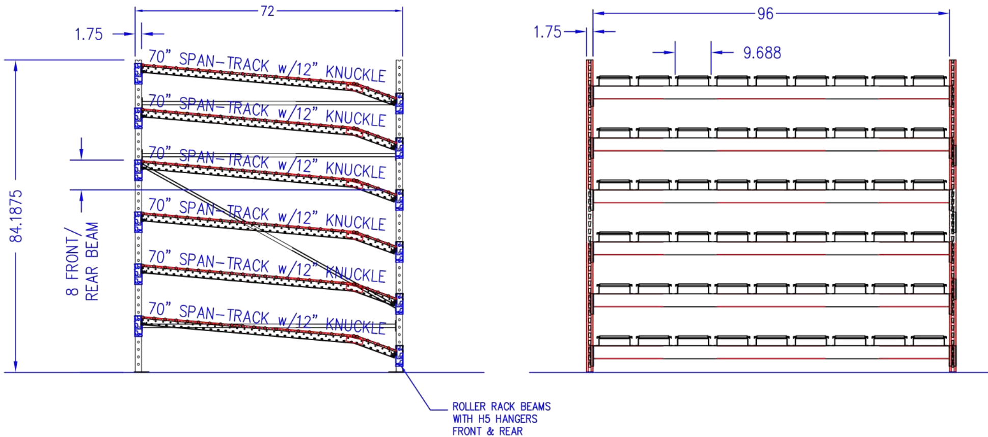
ONE ROLLER RACK UNIT AS SHOWN
